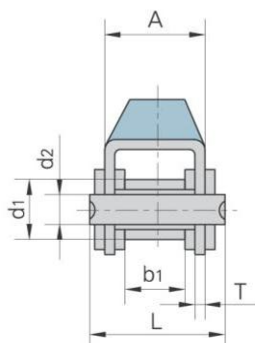
带G1部件 With G1 profile
