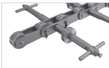
橡胶手套链 Rubber gloves carrier chains
