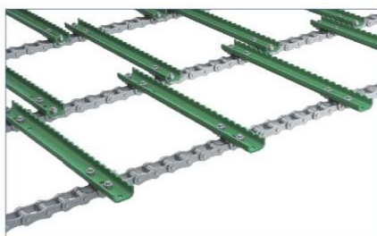
农机喂入链 Agriculture feed chains
