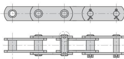
5. 销轴铆头后采用焊接加固 5. Welded pins with plates
