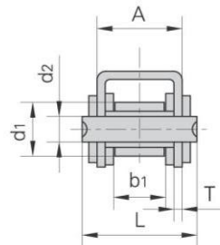
带U1部件 With U1 profile
