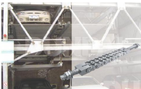
停车库链 Car parking chains
