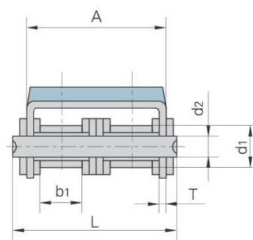
带G2部件 With G2 profile
