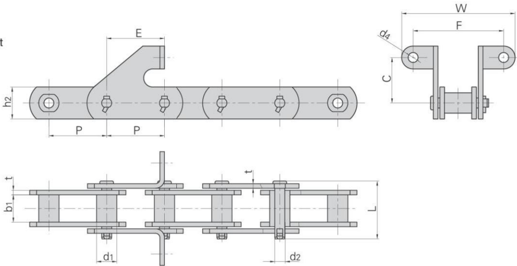
带SD附件 With SD attachment
