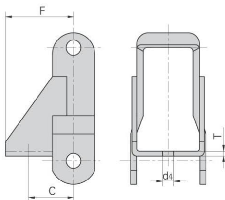
带C1附件 With C1 attachments
