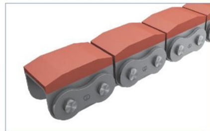
橡胶附板链 Roller chains with elastomer profile
