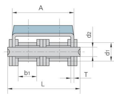
带G2部件 With G2 profile
